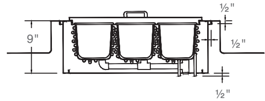
SIDE VIEW: FLAT MOUNTED*
